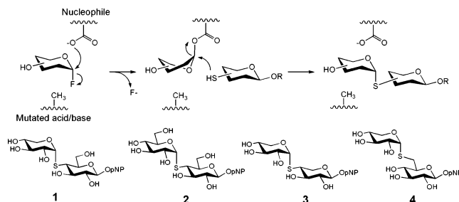
Figure 1. Mechanism of \alpha -thioglycoligases and structures of products.
