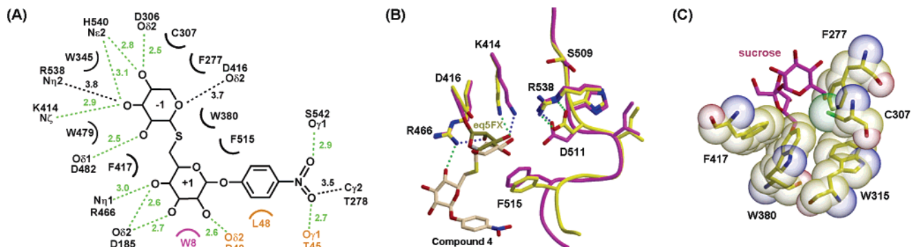
Figure 2. (A) Interactions of YicI with compound 4. Green dotted lines and numbers represent H-bonds and their lengths. Black dotted lines and numbers represent distances between 4 and residues within 4 Å. (B) Superposition of the Michaelis complex (2F2H) and the 5-fluoroxalosyl (eq5FX) enzyme intermediate (1XSK). Side chains for the residues are depicted in bond style coloring with carbon atoms in purple (1XSK) or yellow (2F2H). Hydrogen bonds in 1XSK and 2F2H are represented as blue and green dotted lines, respectively. (C) Modeled structure of YicI with sucrose.
